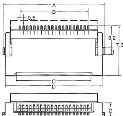
Printed Circuit Board Matching Dimensions (Top View)
