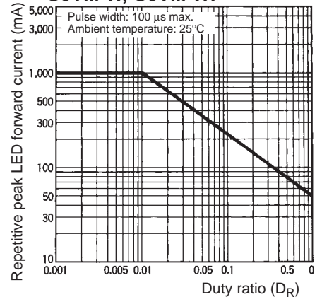
Repetitive Peak LED Forward Current vs. Duty Ratio G3VM-W, G3VM-WF
